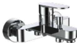
H3315170044001 Bath mixer, fittings distance 134– 166 mm, projection 160 mm, fixed spout, with fittings, without accessories, chrome
